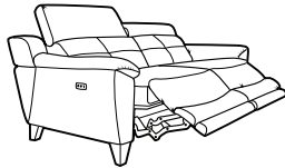
LARGE TWO SEATER POWER RECLINER H100cm (headrest up) H83cm (headrest down) W196cm D103cm SH51cm SW150cm SD57cm AH62cm Fully reclined 160cm
