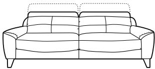
LARGE TWO SEATER SOFA H100cm (headrest up) H83cm (headrest down) W196cm D103cm SH51cm SW150cm SD57cm AH62cm
