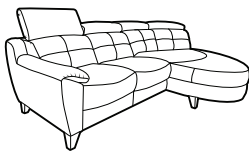
CHAISE END SOFA H100cm (headrest up) H83cm (headrest down) W270cm D179cm SH51cm SW240cm SD57cm AH62cm CSD130cm
