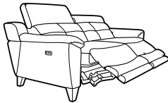
TWO SEATER POWER RECLINER H100cm (headrest up) H83cm (headrest down) W159cm D103cm SH51cm SW115cm SD57cm AH62cm Fully reclined 160cm
