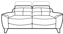
TWO SEATER SOFA H100cm (headrest up) H83cm (headrest down) W159cm D103cmSH51cm SW115cm SD57cm AH62cm
