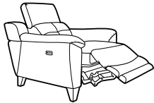
CHAIR POWER RECLINER H100cm (headrest up) H83cm (headrest down) W98cm D103cm SH51cm SW50cm SD57cm AH62cm Fully reclined 160cm
